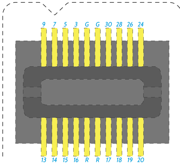
Zif Clip® Connector (Looking through clip)
